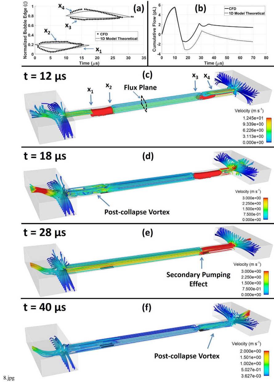
FIG. 8. Contactless Bubble-bubble Interaction \tau = 10 \mu s , \xi_{o,1} = 0.2 , \xi_{o,2} = 0.8 , L = 500 \mu m . (a-b) describe one-dimensional model data overlaid on FLOW-3D CFD data. (a) depicts the bubble edges over time and (b) depicts the cumulative flow through the microchannel over time. Resistor placement and firing delay were \xi_{o,1} = 0.2 , \xi_{o,2} = 0.8 , and \tau = 10 \mu s with a one-dimensional model bubble strength of q_o = 4.26 \times 10^{-10} kg/m.s . (c-f) illustrates 3D CFD flow structures and bubble dynamics. (c) shows initial bubble expansion, (d) shows the first post-collapse vortex formation, (e) showcases the momentum imbalance between fluid legs giving rise to the secondary pumping effect, and (f) shows the second post-collapse vortex formation. Bubble edges are labeled x_{1-4} and net flow was measured at the flux plane.
