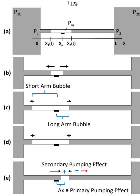
FIG. 1. Schematic of the Inertial Pump 1D Model. (a) Depicts a microchannel with two fluid reservoirs of pressure p_{1b,2b} and channel inlet/outlet pressure p_{1,2} . At its simplest case, p_{1b,2b} = p_o and the fluid starts at rest. (b-e) describes the pumping process. (b) Local boiling generates a high pressure vapor bubble, p_{vr} , that pushes fluid out of the channel. (c) p_{vr} decreases due to bubble volumetric expansion and heat transfer and rapidly drops below atmospheric pressure to p_{vr} . Bubble expansion is driven by inertia until the bubble reaches its maximum expansion volume. (d) The short arm bubble (to the left of the resistor) reverses direction while the long arm bubble (to the right of the resistor) continues expanding to the right. (e) The short arm bubble accelerates faster than the long arm bubble resulting in a momentum imbalance that drives fluid flow upon collapse. The point of collapse is offset from the location of bubble expansion giving rise to the primary pumping effect . The net momentum imparted to the fluid generates the secondary pumping effect which is eventually brought to rest by viscous dissipation.
